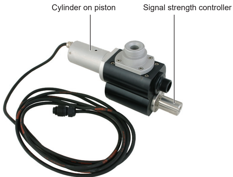
Fig. 16: Stopper
