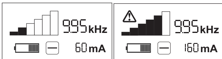
Fig. 7: Energizing for electromagnetic location – main view Left image: Signal strength in ES1 range (safe-to-touch range) Right image: Signal strength in ES2 range ( Notice symbol)
